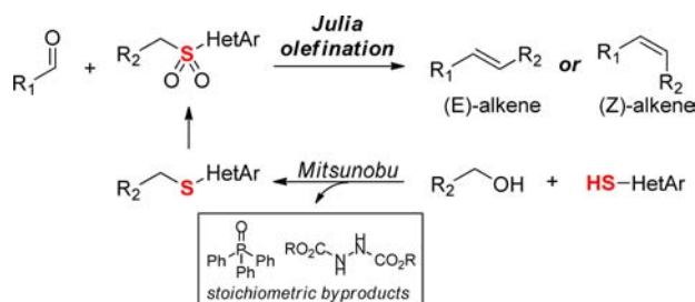
Scheme 1. Alkene Synthesis by Julia Olefination
