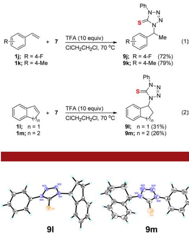
Figure 1. X-ray crystal structure of 9l and 9m .
